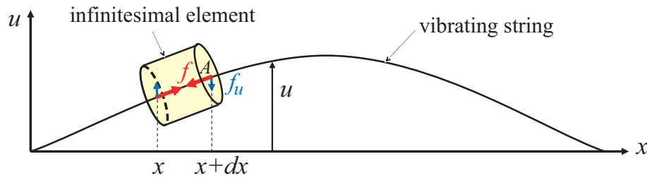
Figure 8.1: Applying Newton's second law of motion to an infinitesimal element of a string yields the 1-d wave equation u_{tt} = c^2 u_{xx} .
