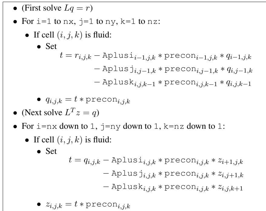
Figure 4.3: Applying the MIC(0) preconditioner in three dimensions ( z = Mr ).
